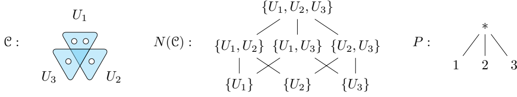
FIGURE 1. A strong combinatorial cover
